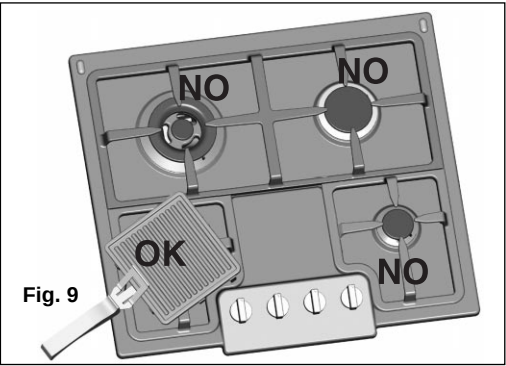
Fig 9 - Positioning of griddle when in use
